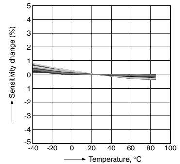
3-1 Sensitivity temperature characteristics X-axis (VDD=5V)
