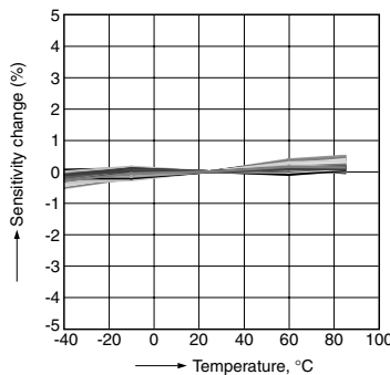
3-2 Sensitivity temperature characteristics Y-axis (VDD=5V)
