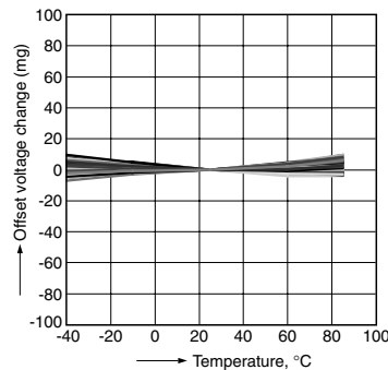
4-1 Offset voltage temperature characteristics X-axis (VDD=5V)
