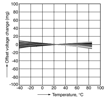
4-2 Offset voltage temperature characteristics Y-axis (VDD=5V)
