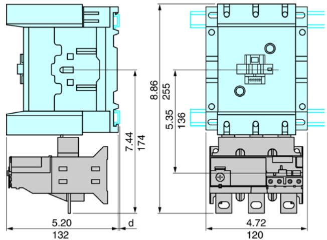
LR9D Direct mounting beneath contactors LC1D115 and D150
