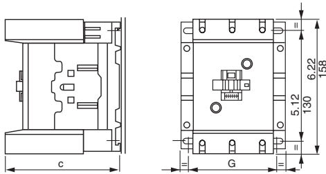
LC1D115, D150 Panel mounted with 1/4" screws
