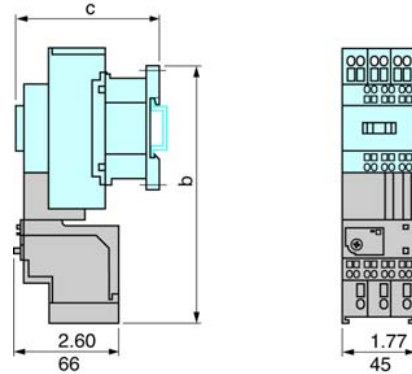
LRD-013-353 Direct mounting beneath contactors with spring terminal connections
