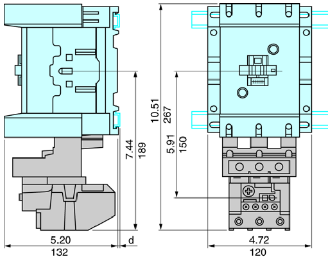
LRD4*** Direct mounting beneath contactors LC1D115 and D150
