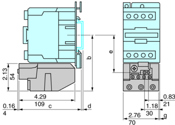
LRD-3*** Direct mounting beneath contactors LC1-D40 to D95 and LP1-D40 to D80
