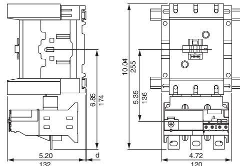
LR9D solid-state overload relay Direct mounting beneath contactors LC1D115 and D150
