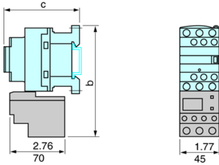
LRD-01-35 Direct mounting beneath contactors with screw
