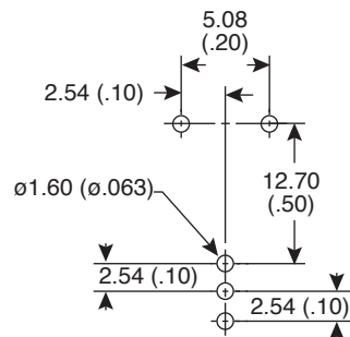
Mounting Holes
