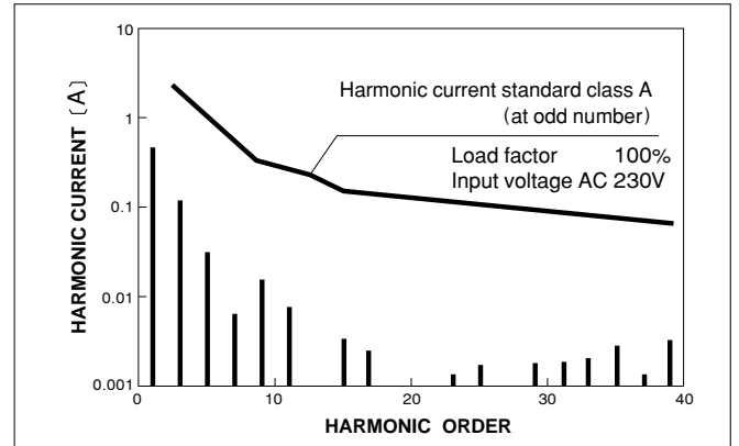
INPUT HARMONIC CURRENT (LEA75F-5)
