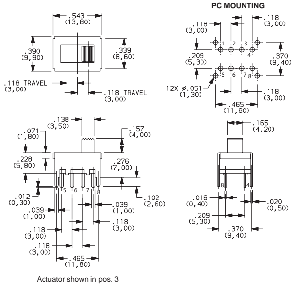
OS203013MT6QN1 DP3T
