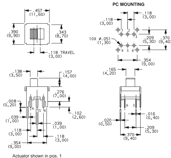
OS202013MT5QN1 DPDT
