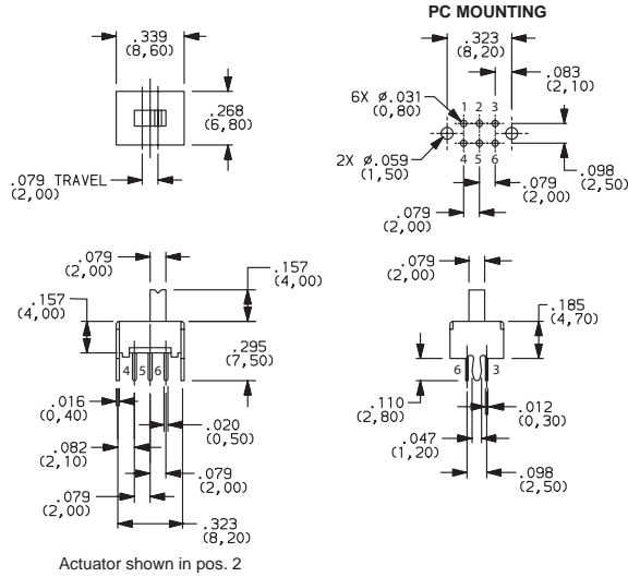
OS202011MS2QS1 DPDT
