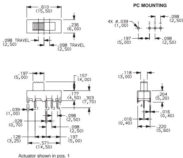
OS103012MU2QP1 SP3T
