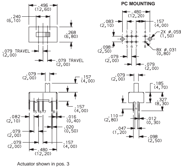
OS203011MS1QP1 DP3T
