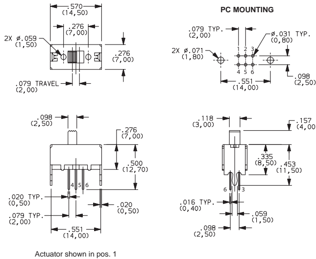
OS202011MV4QN1 DPDT
