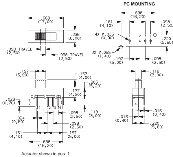
OS103012MU1QP1 SP3T
