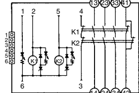
G9SA-EX301
