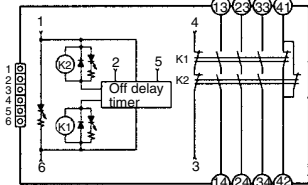
G9SA-EX031-T
