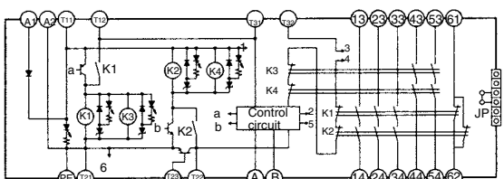
G9SA-501 (24 VAC/VDC)
