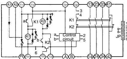
G9SA-301 (24 VAC/VDC)
