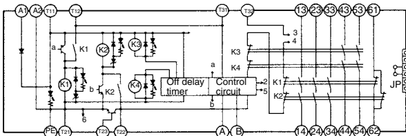
G9SA-321-T (24 VAC/VDC)
