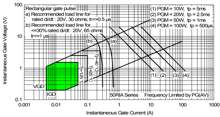
Fig. 16 - Gate Characteristics
