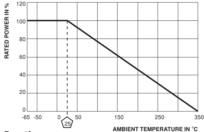
Derating
