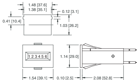
Mounting hole: For M3 screw
