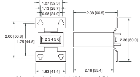
Mounting holes: 0.14" [3.6mm] Dia.
