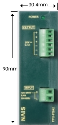
FP0 Power supply FP0-PSA2
