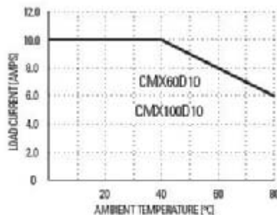
Max. Load Current vs. Temp.
