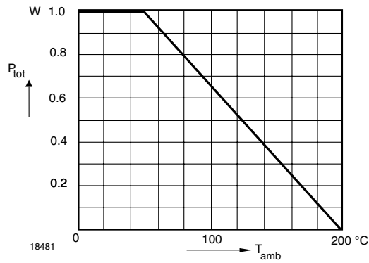
Figure 1. Admissible Power Dissipation vs. Ambient Temperature
