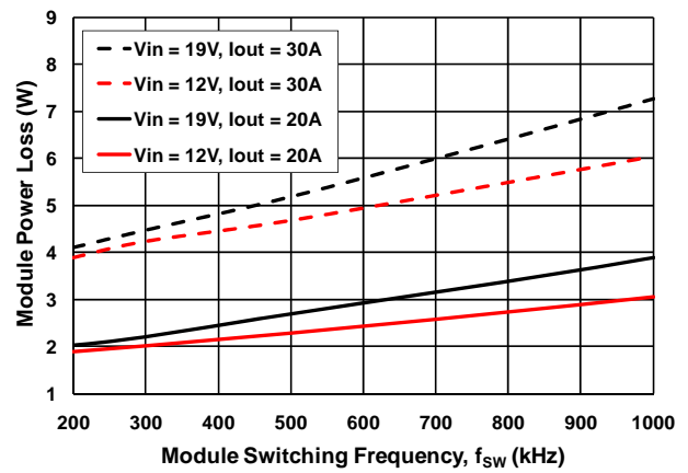
Figure 9. Module Power Loss vs. Switching Frequency
