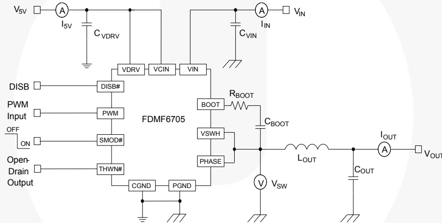
Figure 28. Power Loss Measurement Block Diagram
