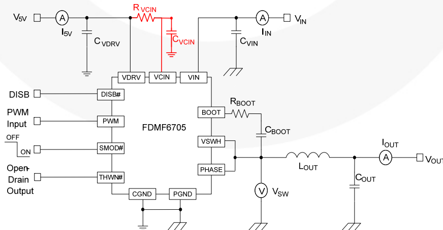
Figure 29. Block Diagram with VCIN Filter
