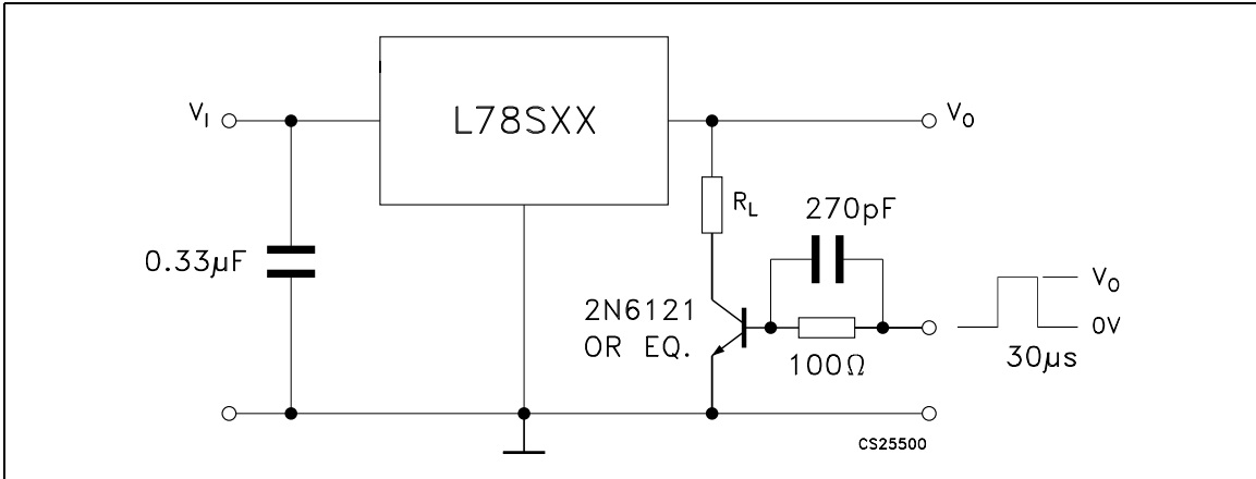
Figure 6. Load regulation
