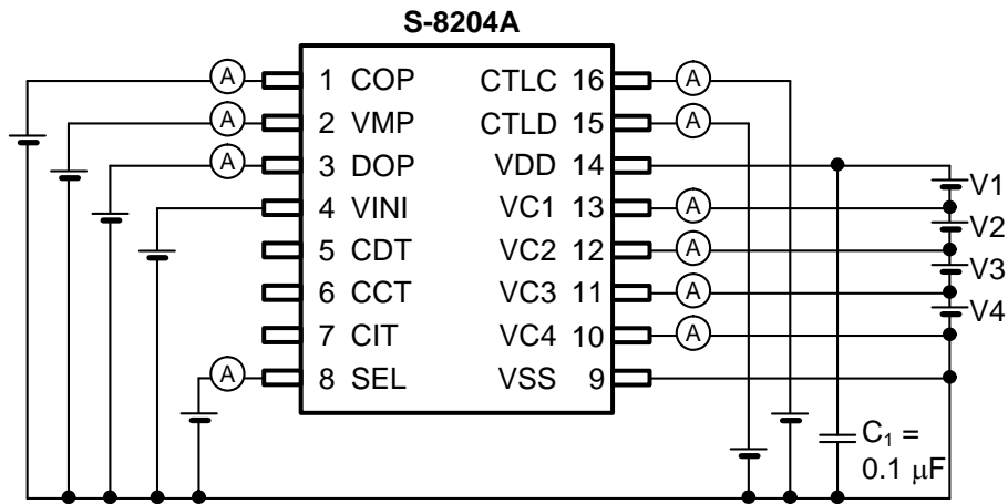
Figure 8 Test Circuit 5
