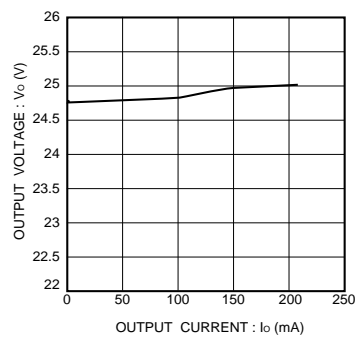
Fig.15 Output characteristic
