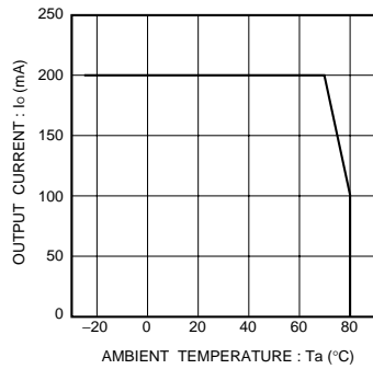
Fig.9 Derating curve
