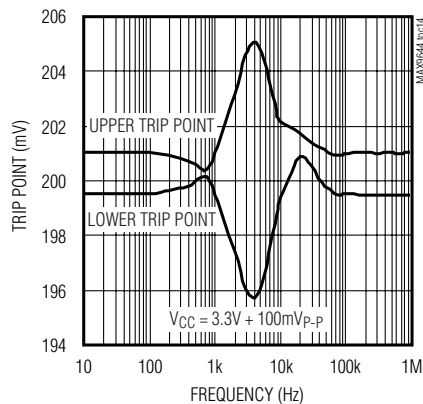
POWER-SUPPLY REJECTION FOR NO FALSE TRIGGERING
