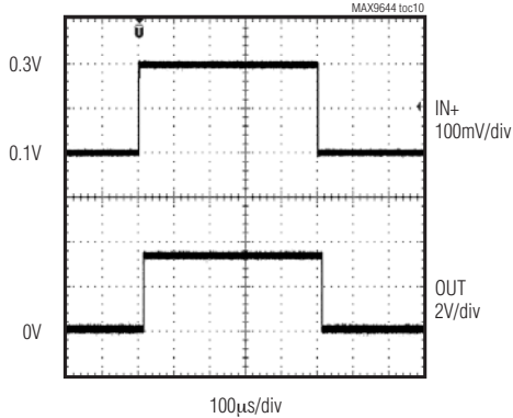
PROPAGATION DELAY AT V_{CC} = 3.3V
