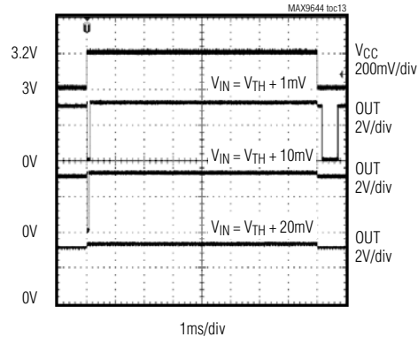
OUTPUT RESPONSE TO SUPPLY VOLTAGE TRANSIENT
