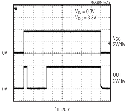
POWER-UP/POWER-DOWN RESPONSE
