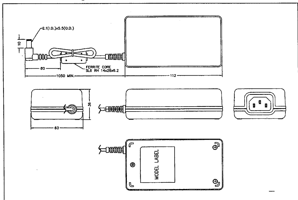
Dimension Diagram Unit: mm (inch)
