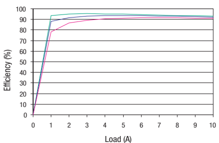
V_{OUT} = 2.5V
