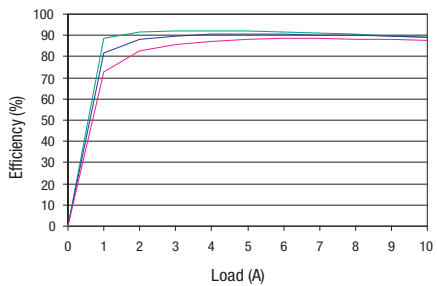
V_{OUT} = 1.8V
