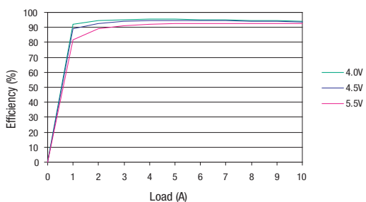
V_{OUT} = 3.3V
