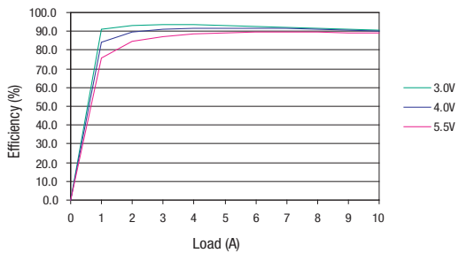
V_{OUT} = 2.0V
