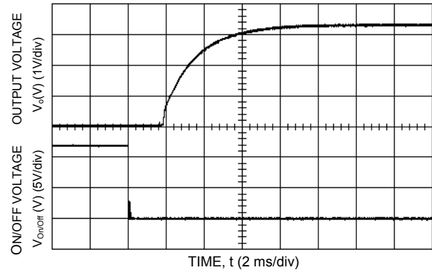
Figure 4. Typical Start-Up Characteristics from Remote ON/OFF.
