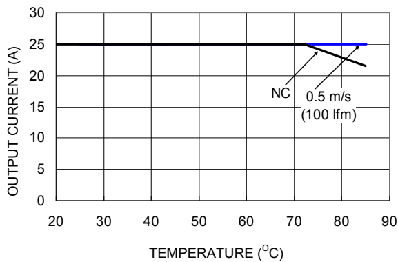
Figure 16. Thermal Derating Curves for the QPW025A0F41-H baseplate module at 48Vin. Airflow is in the transverse direction (Vin- to Vin+).
