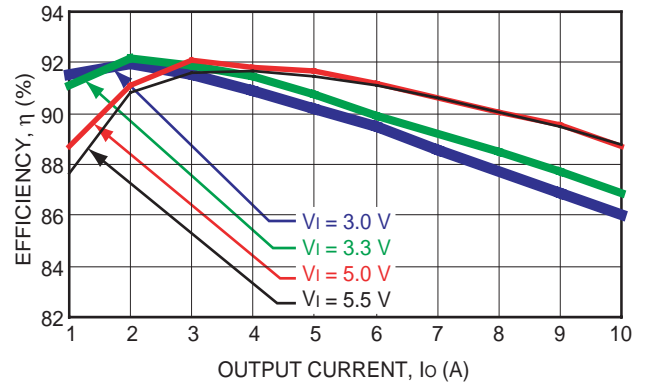
Figure 6. Converter Efficiency vs output current AXH010A0M-SR(1.5V Output Voltage).
