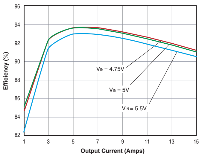
UNR-3.3/20-D5 Efficiency vs. Load @ 25°C Ambient
