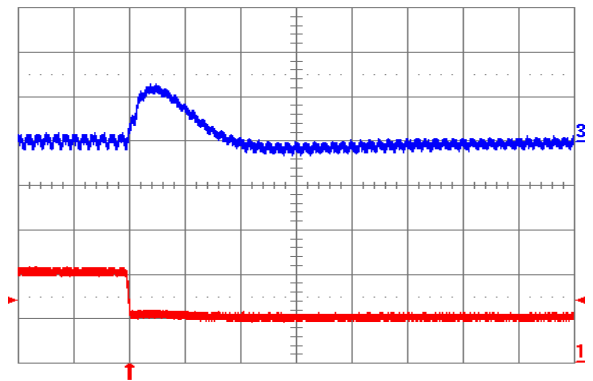
Fig. 1.8V.8: Output voltage response for V_{out} = 1.8 V to negative load current step change from 10 A to 5 A with slew rate of -5 A/ \mu s at V_{in} = 12 V. Top trace: output voltage (100 mV/div.); Bottom trace: load current (5 A/div.). C_o = 100 \mu F ceramic. Time scale: 20 \mu s/div.
