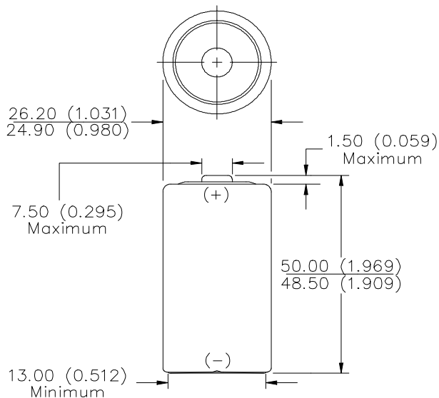
Industry Standard Dimensions in mm (inches)
