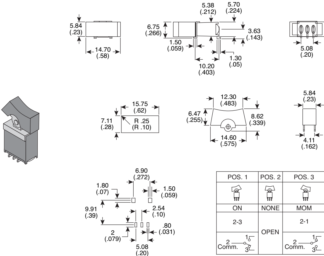
P.C. MOUNTING
