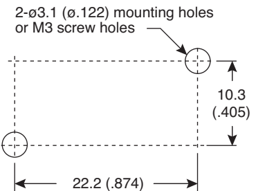
Mounting Holes
