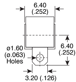
Solder Terminal
