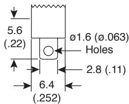
Solder Terminals
