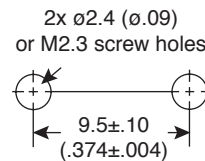
Mounting Holes
