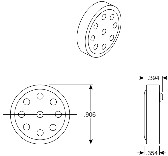
Dimensions (In.)
