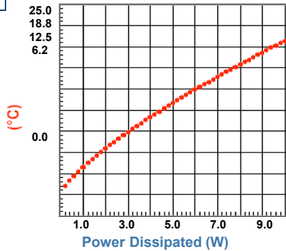
Heat Sink Temperature Rise Above Ambient
