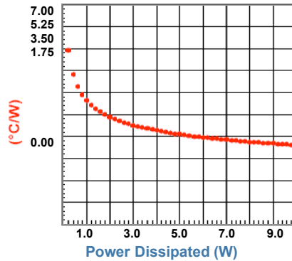
Heat Sink Thermal Resistance
