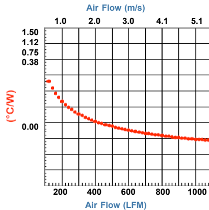
Heat Sink Thermal Resistance
