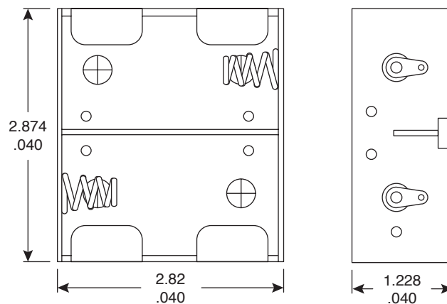
Dimensions: In.
