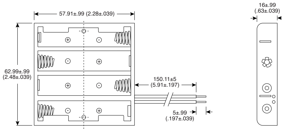
Dimensions: mm (In.)
