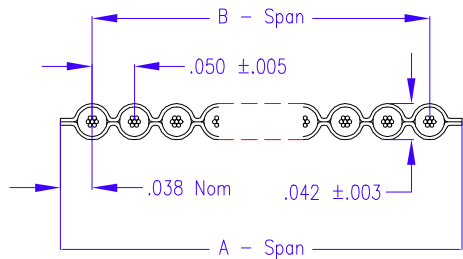
Cross Section at Flat
