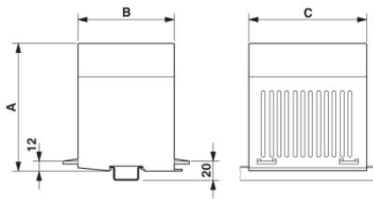
Dimension A=165 mm; dimension B=149 mm; dimension C=200 mm
