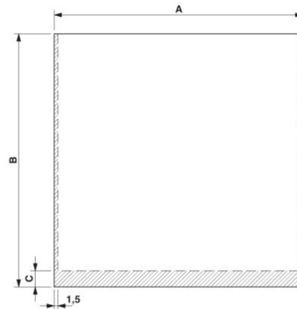
PCB 8, 13: Dimension A: 141.0 mm; B: 140.5 mm; C: 0 mm
