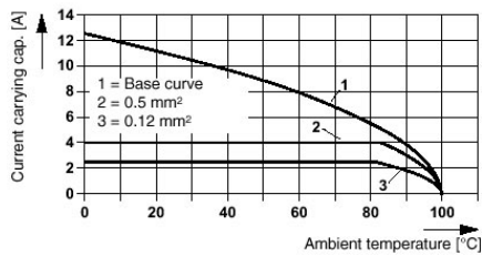
FK-MPT 0,5-ST-3,5 with PST 1,0
