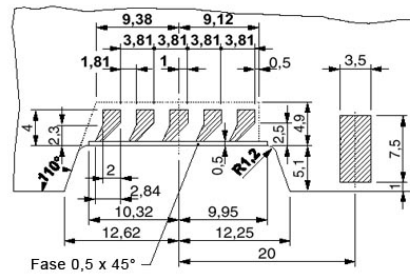
Detailed dimensional drawing of the DIN rail connector contact pads
