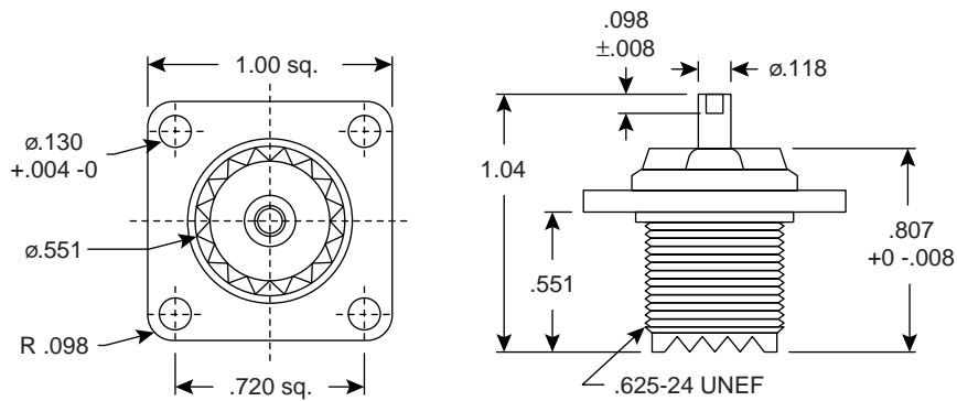
Dimensions (In.)
