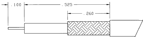
CABLE STRIPPING DIMENSIONS
