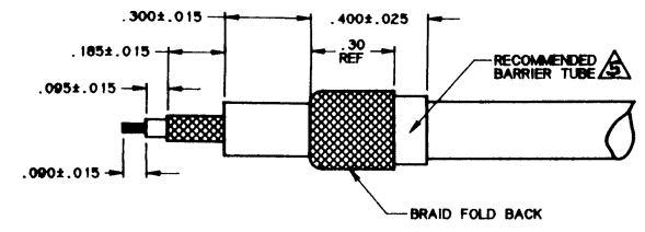
TRIAx STRIP (RAYTHEON #10270730)
