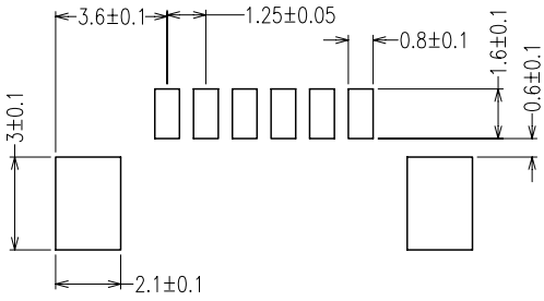
PCB LAYOUT SURFACE MOUNTING
