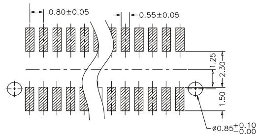
Plug or Socket PCB LAYOUT
