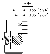
SECTION W-W
