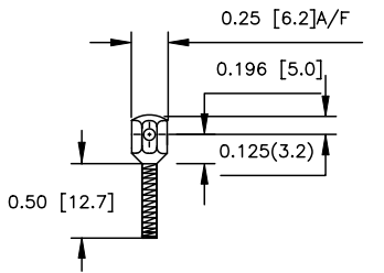
SCREW 6 BA Brass, Nickel Plated
