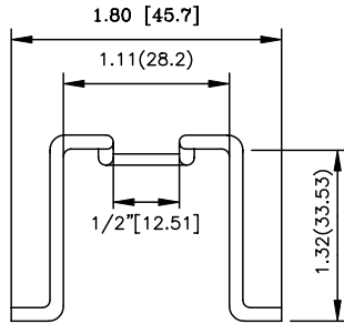
CLIP .072" Dia. Stainless Steel Wire
