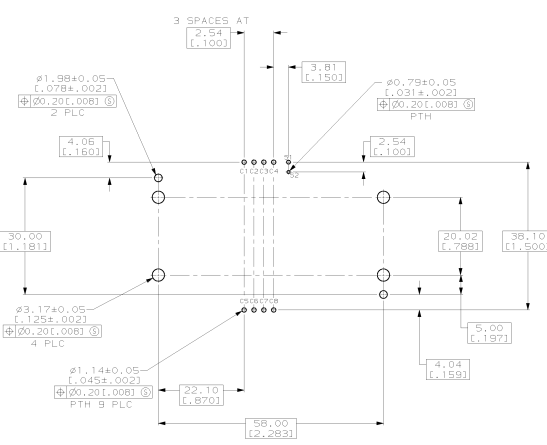
RECOMMENDED P.C.B. LAYOUT PCB THICKNESS 1.57 [0.062]
