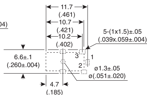
FOOT PRINT (BOTTOM VIEW)
