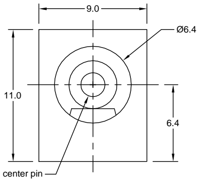
Recommended PCB Layout (Bottom View)
