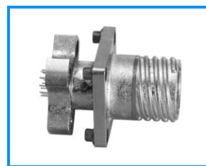
Composite shell stand-off Filter 38999 connector
