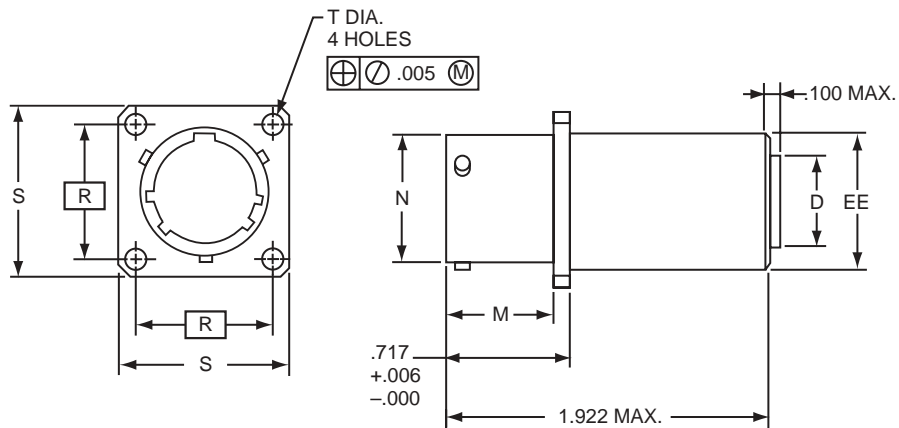
21-65X2XX-XXX UTS (Crimp) Contact MIL-C-39029/57
