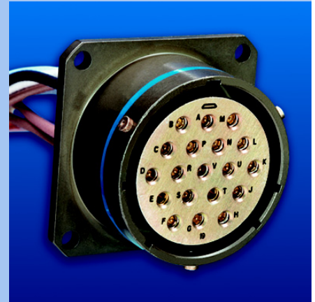
Ground Plane Connector with Metallic Insert and Concentric Twinax Contacts
