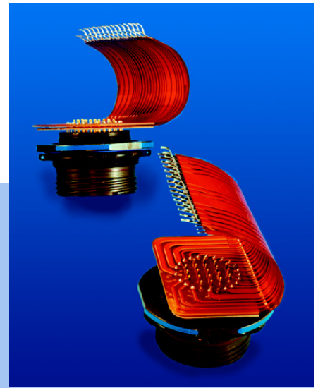
D38999 Connectors with PCB Tail Twinax Contacts
