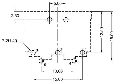
Recommended PCB Layout (Bottom View)
