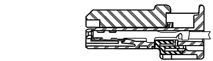
CONTACT ASSEMBLY CONDITION (REF.) 端子組込後状態図(参考)
